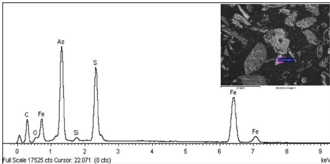
Figure 20. SEM-EDS of the typical arsenopyrite grain found.
