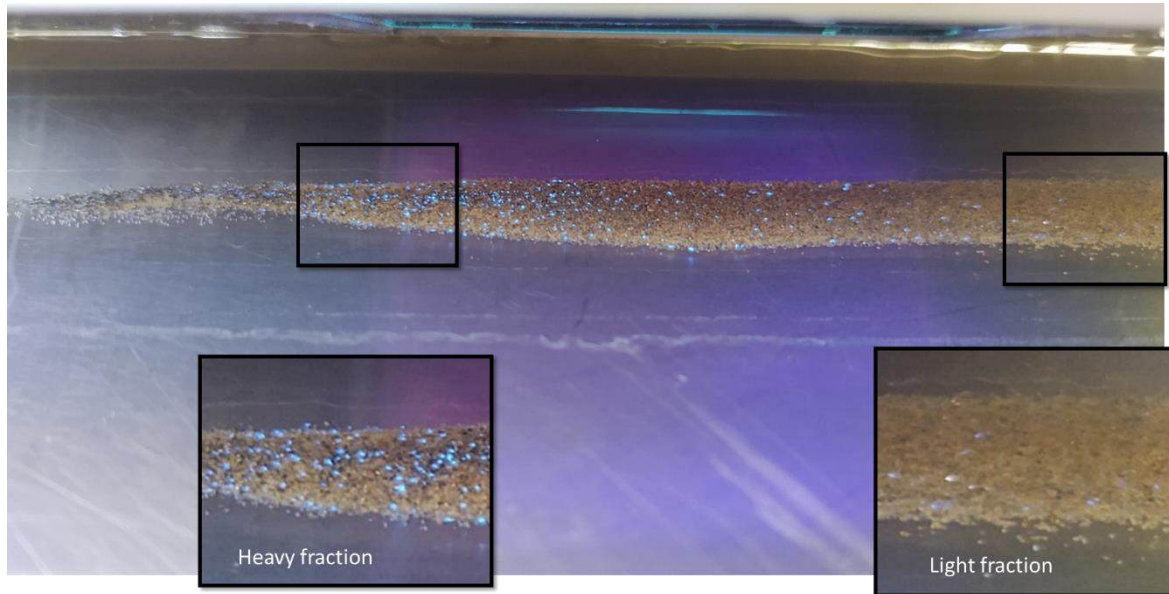
Figure 9. Observation under UV shortwave of heavy and light fractions from 250-500 µm fraction recovered by Mozley shaking table (blue bright spots correspond to scheelite minerals).
