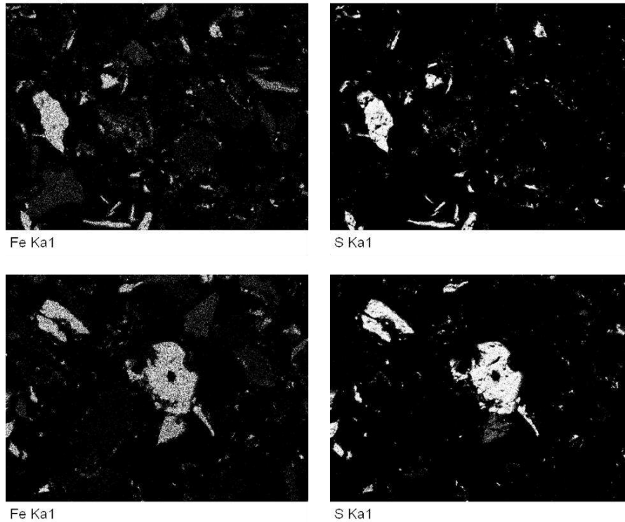
Figure 19. SEM-EDS of Fe and S for two different regions of the W-tailings concentrate CC1.
